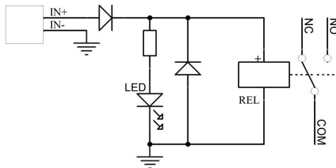
Fig.2. Electrical diagram.
